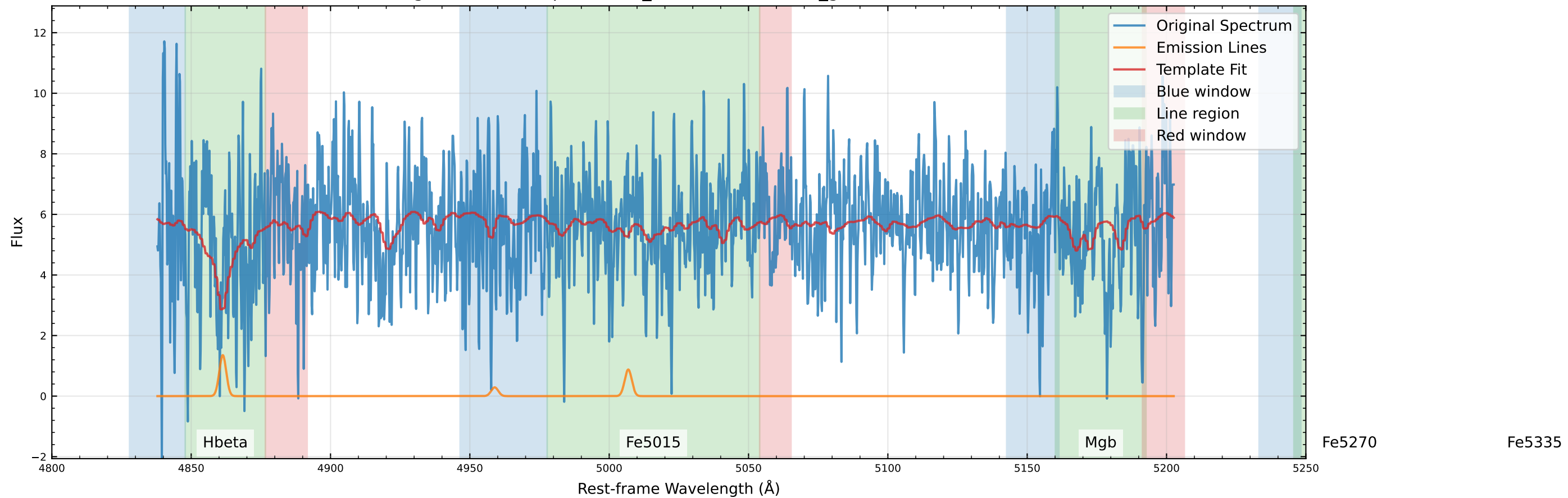
Original Data Comparison (v_star=-84.8 km/s, v_gas=79.9 km/s)
