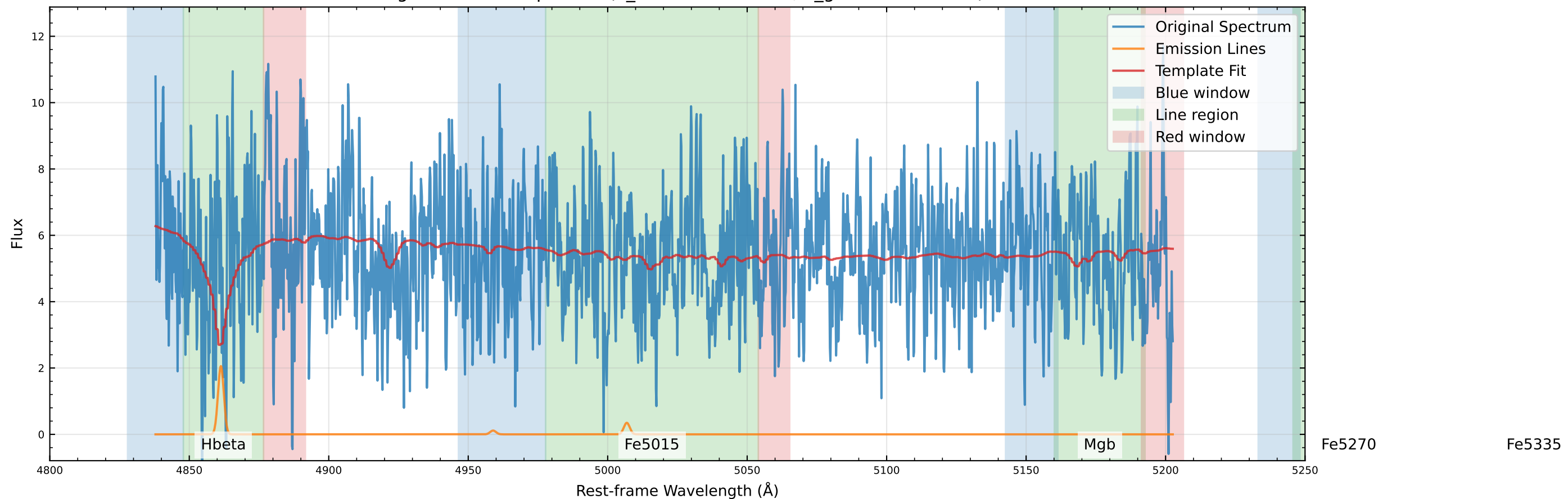
Original Data Comparison (v_star=-226.3 km/s, v_gas=-214.0 km/s)
