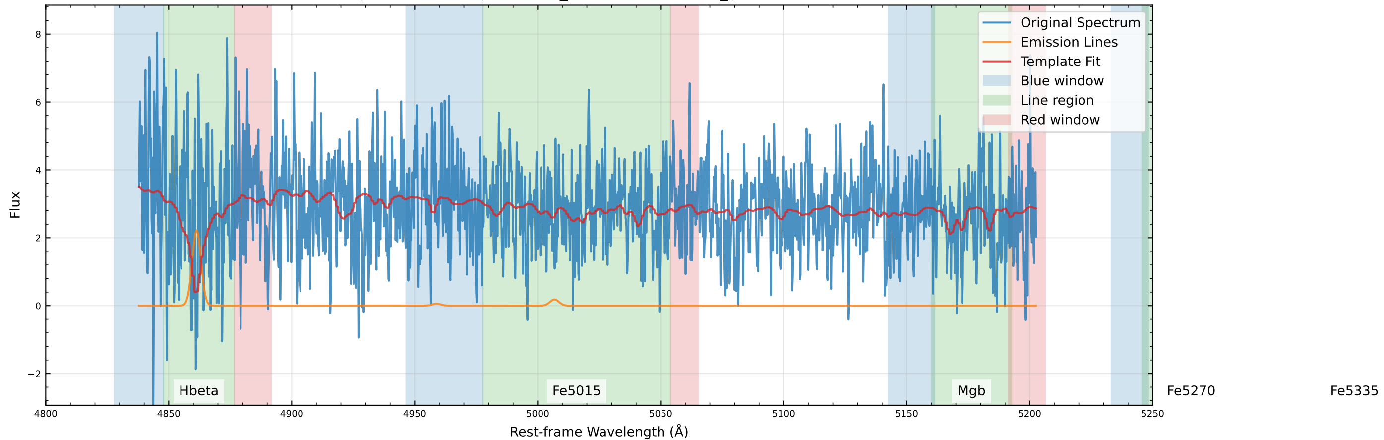
Original Data Comparison (v_star=176.4 km/s, v_gas=192.4 km/s)
