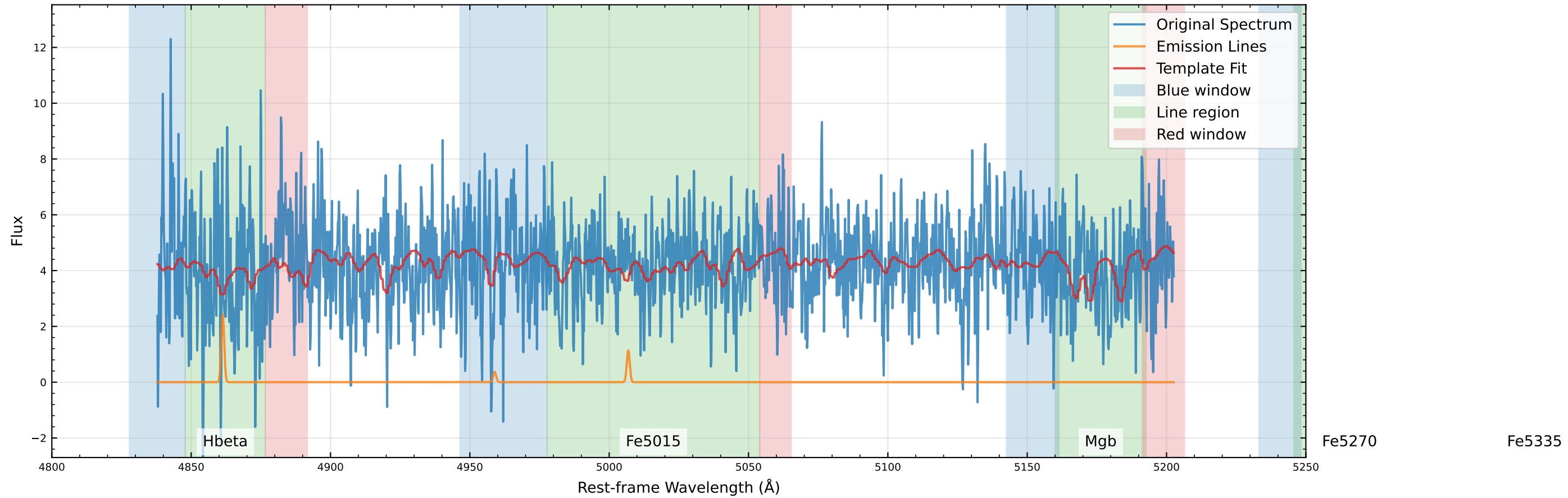
Original Data Comparison (v_star=-215.6 km/s, v_gas=-126.1 km/s)
