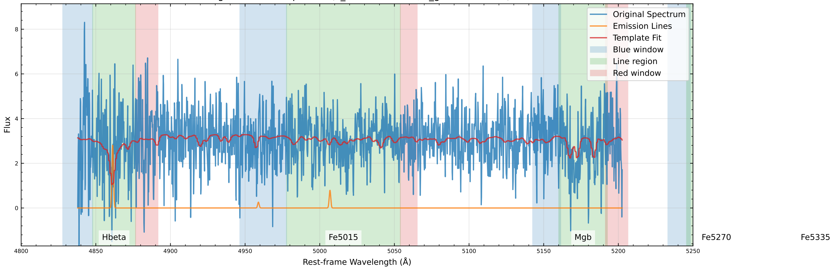
Original Data Comparison (v_star=-3.1 km/s, v_gas=58.5 km/s)
