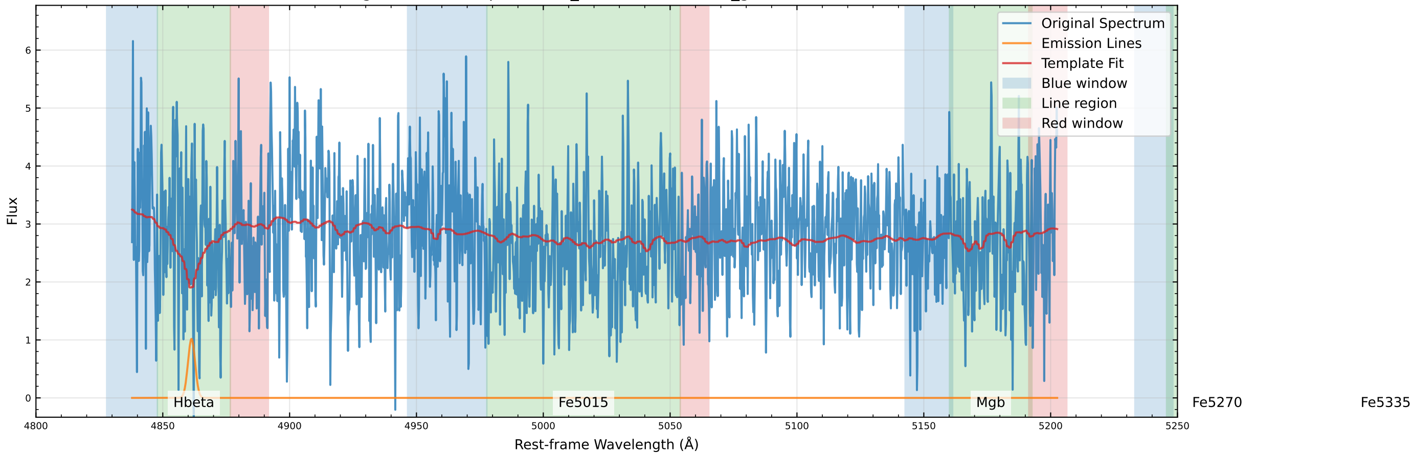
Original Data Comparison (v_star=-70.7 km/s, v_gas=-23.2 km/s)
