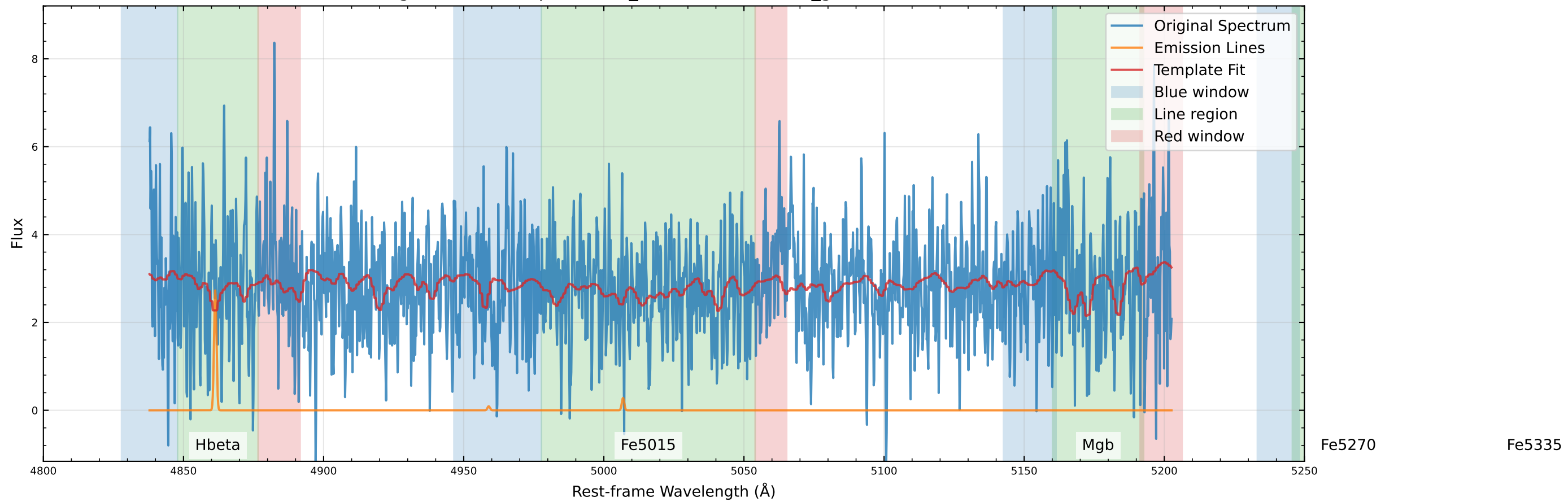
Original Data Comparison (v_star=237.2 km/s, v_gas=197.8 km/s)
