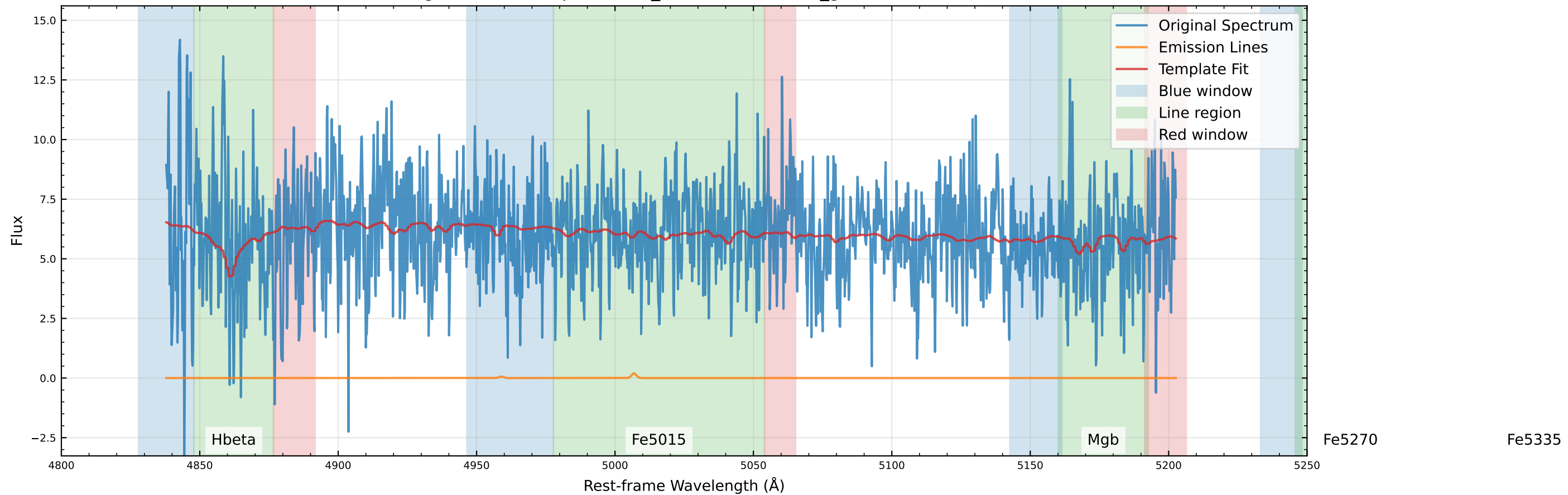
Original Data Comparison (v_star=52.2 km/s, v_gas=46.3 km/s)
