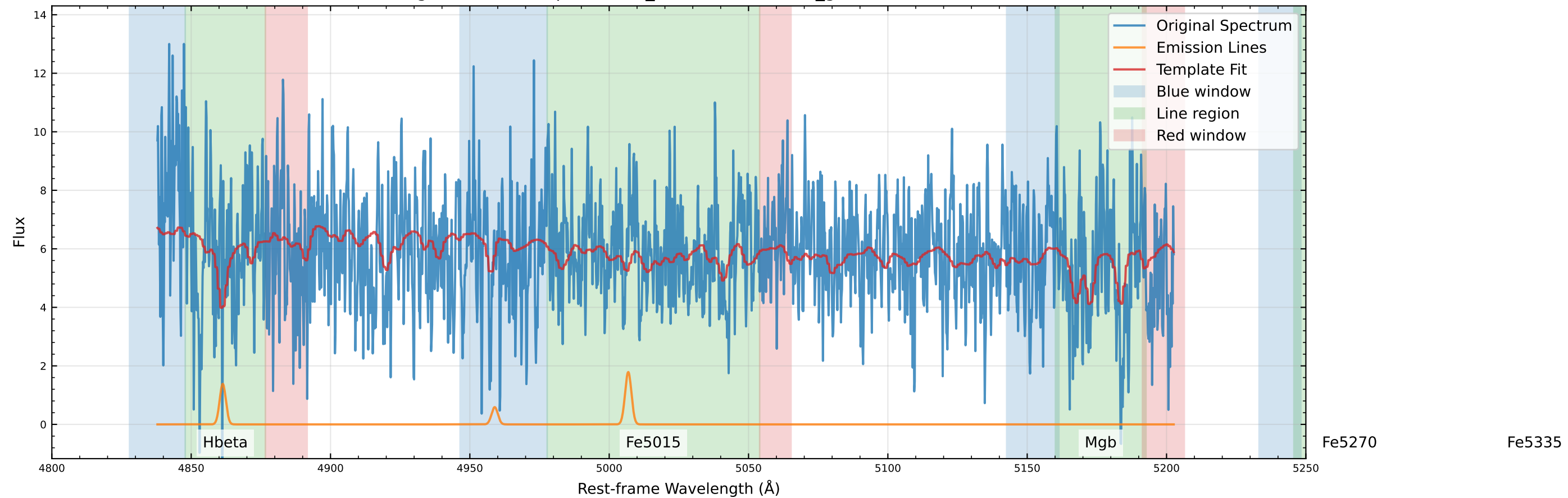
Original Data Comparison (v_star=12.9 km/s, v_gas=60.4 km/s)
