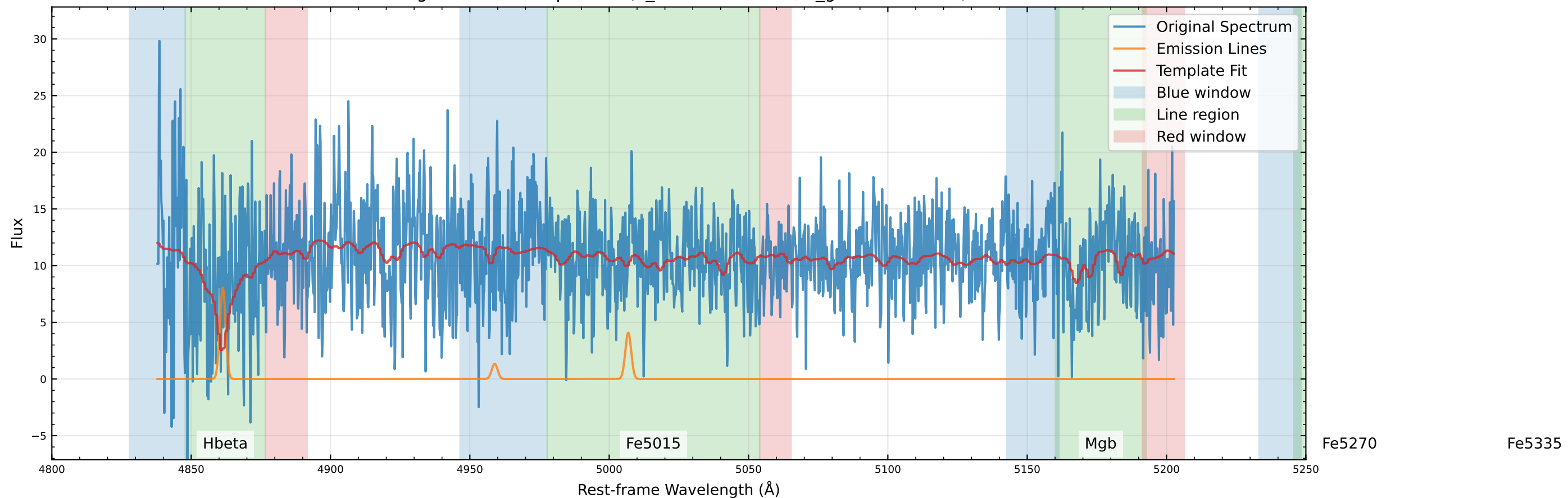
Original Data Comparison (v_star=48.2 km/s, v_gas=34.8 km/s)
