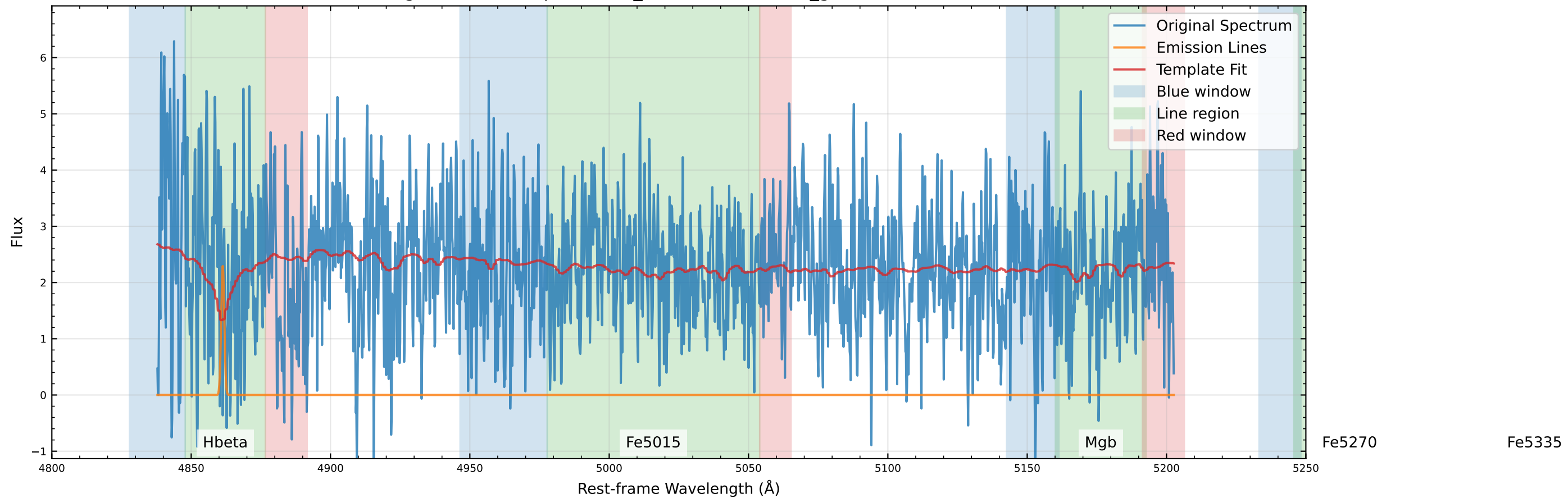
Original Data Comparison (v_star=-49.1 km/s, v_gas=-153.2 km/s)
