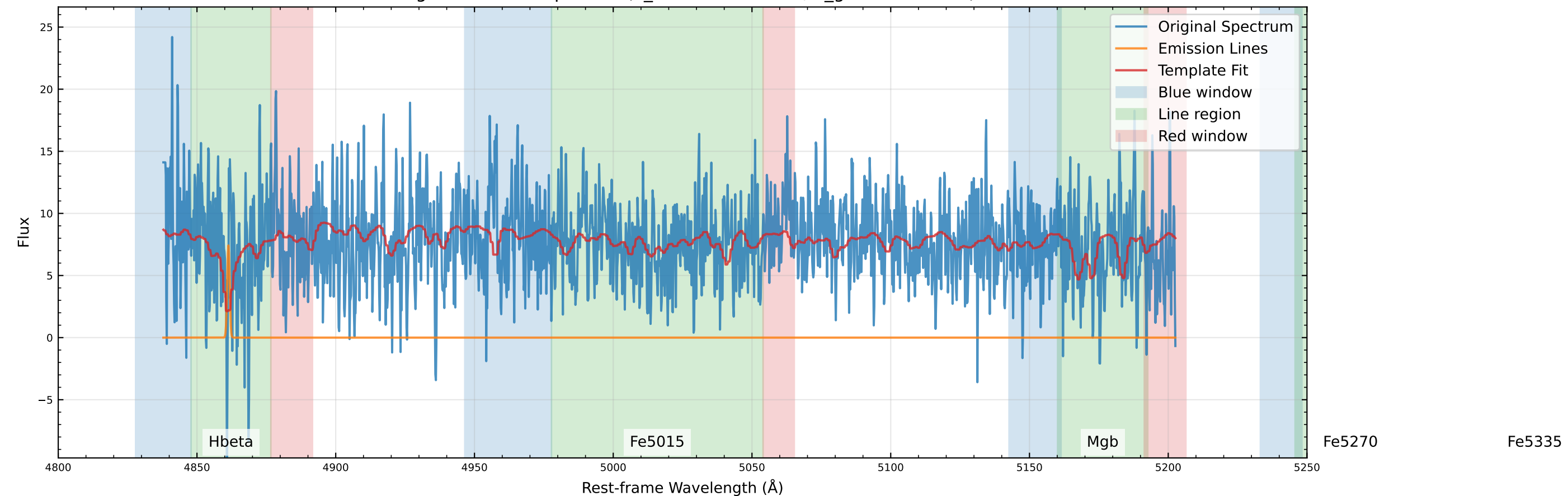
Original Data Comparison (v_star=100.9 km/s, v_gas=39.3 km/s)
