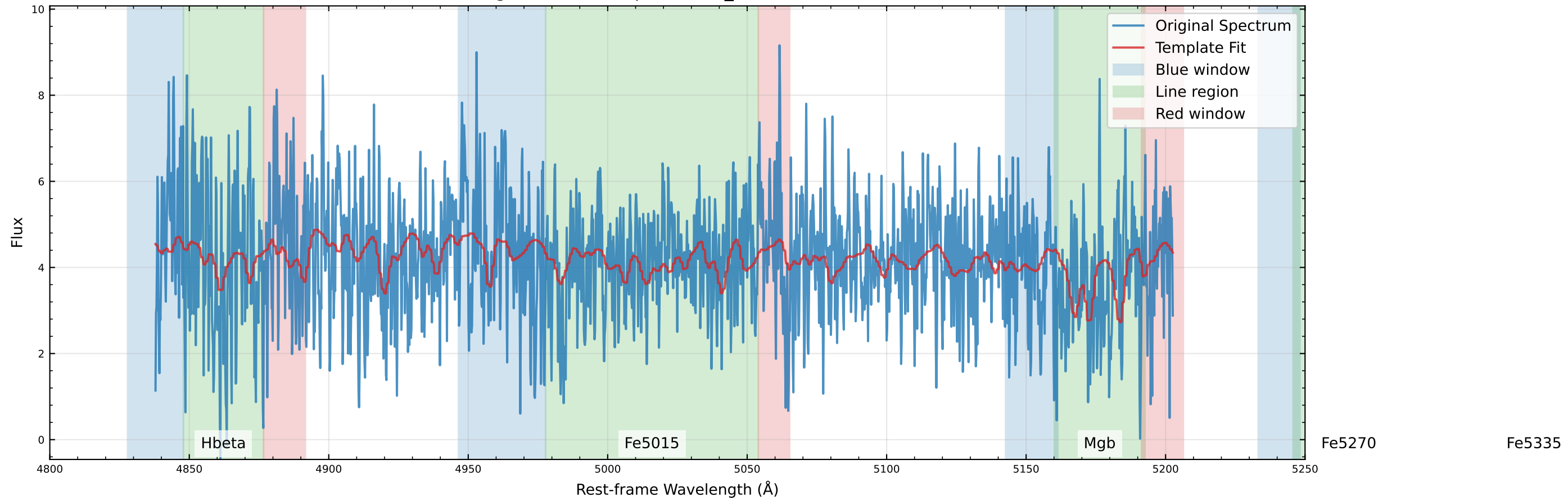
Original Data Comparison (v_star=-80.5 km/s)
