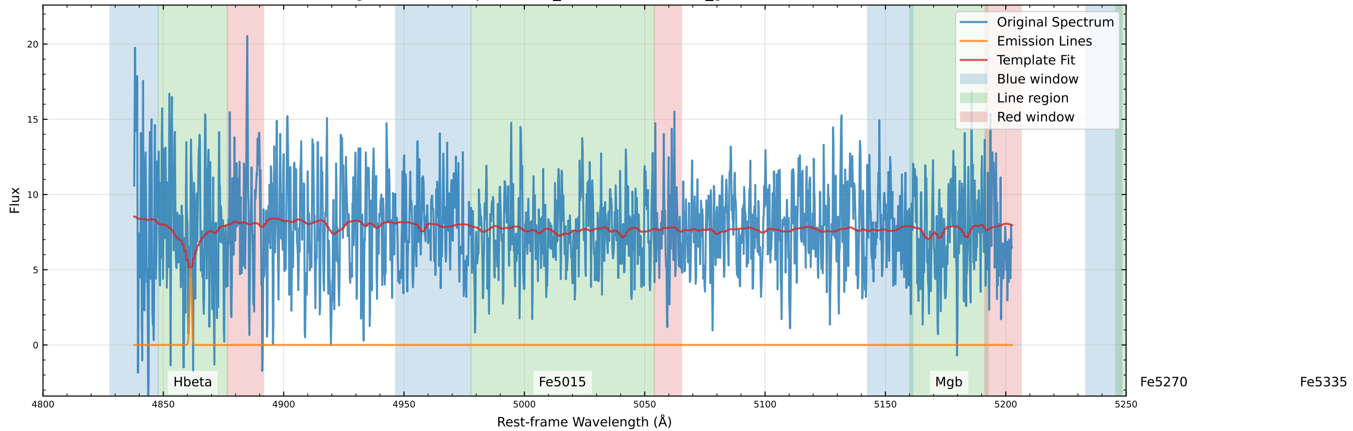
Original Data Comparison ( v_{\text{star}}=-18.0 km/s, v_{\text{gas}}=12.9 km/s)
