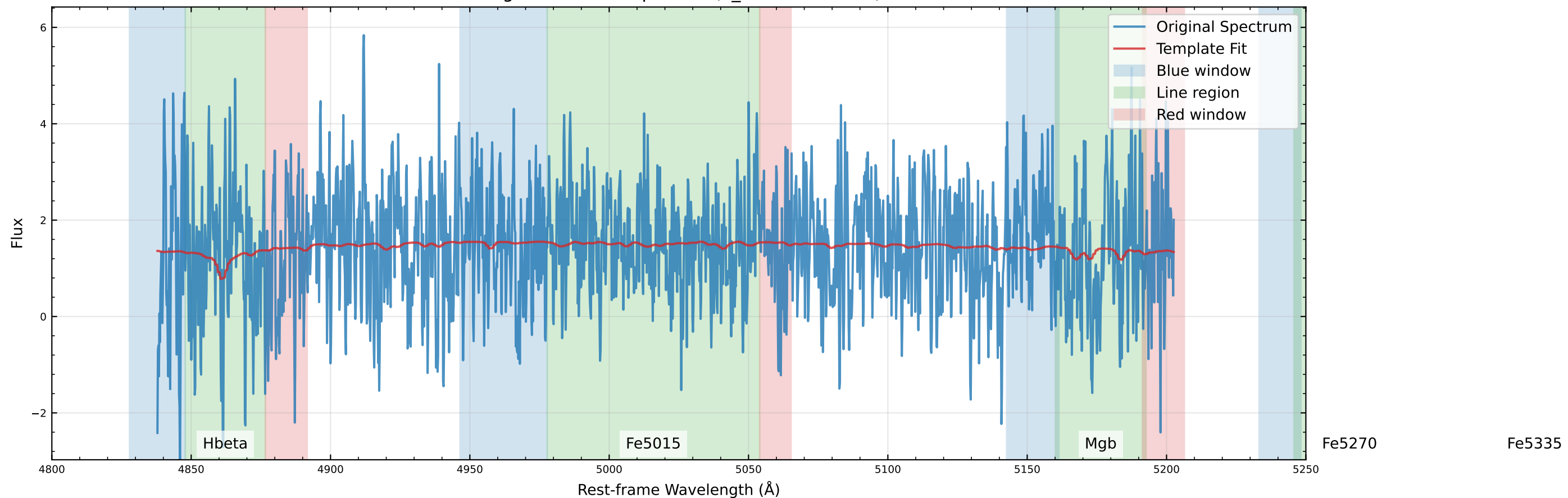
Original Data Comparison (v_star=-2.0 km/s)
