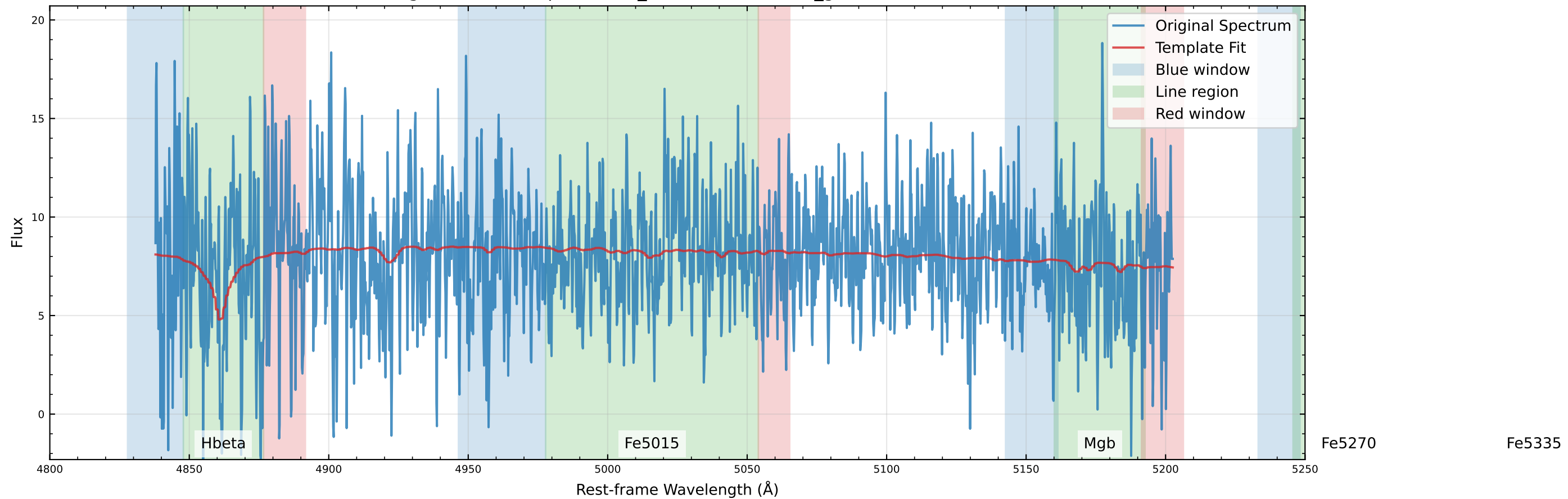
Original Data Comparison (v_star=-55.7 km/s, v_gas=-53.8 km/s)
