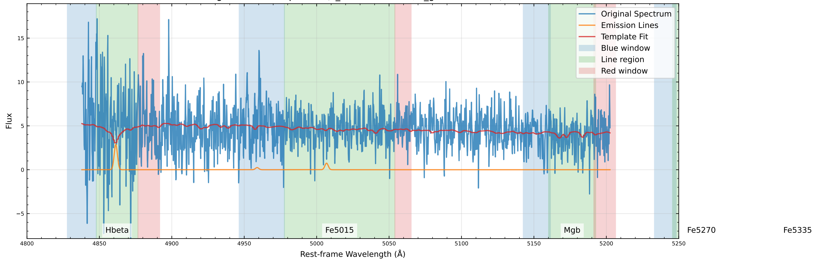
Original Data Comparison (v_star=47.0 km/s, v_gas=61.3 km/s)
