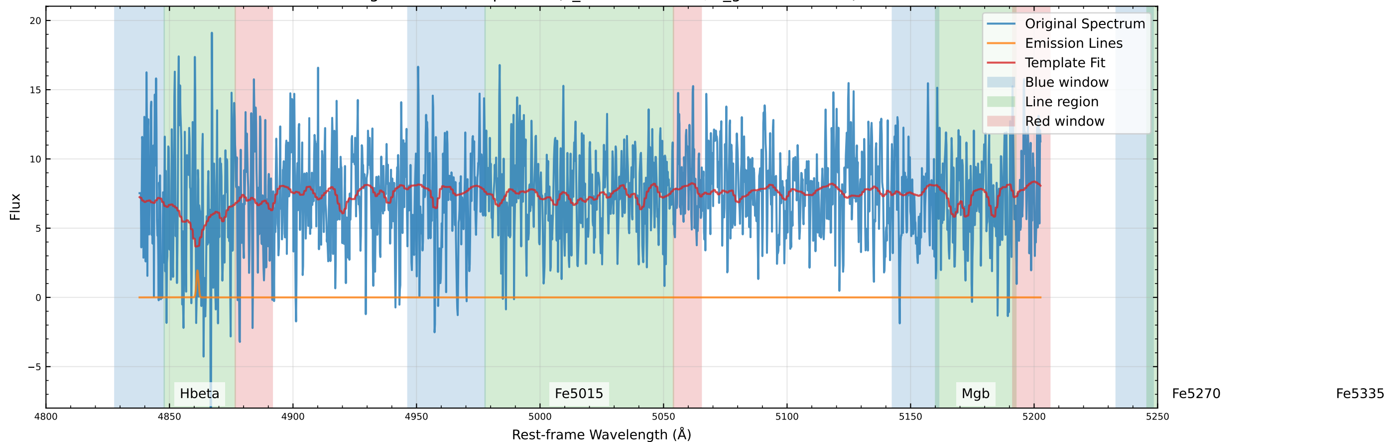
Original Data Comparison (v_star=70.8 km/s, v_gas=37.8 km/s)
