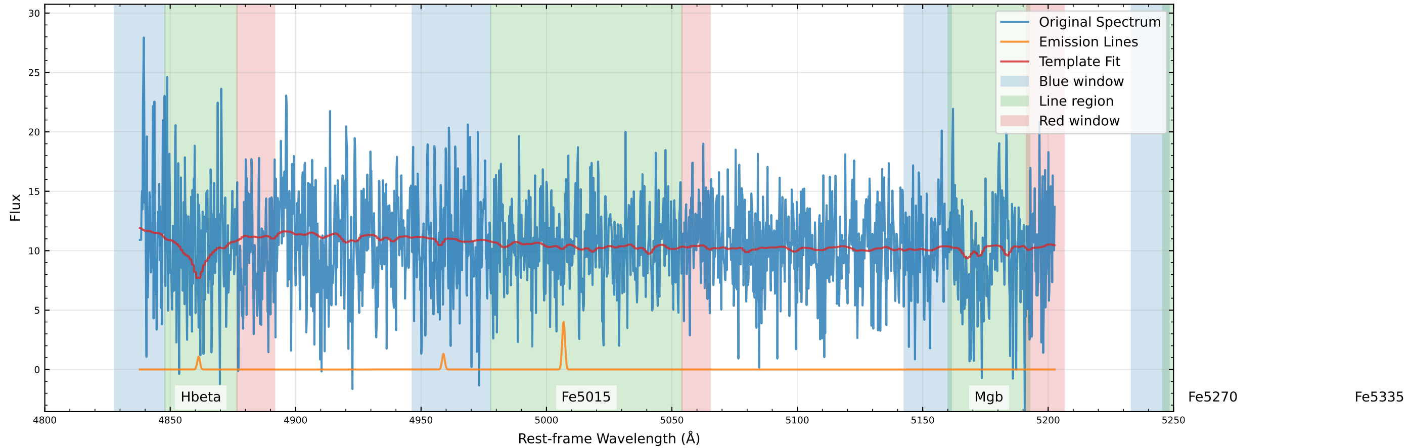
Original Data Comparison (v_star=65.9 km/s, v_gas=72.9 km/s)
