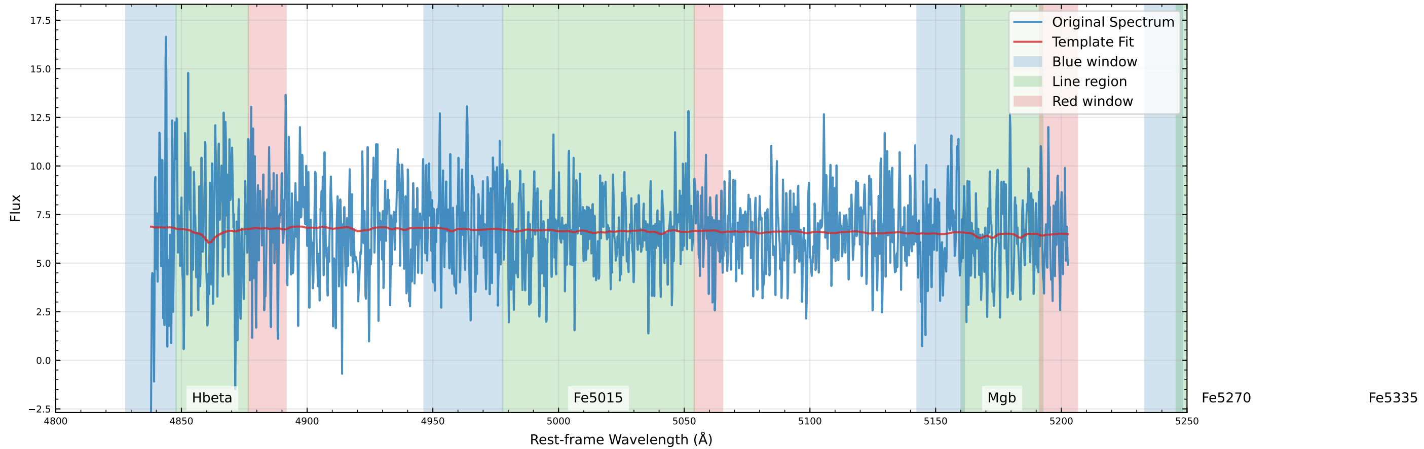
Original Data Comparison (v_star=-1.5 km/s)
