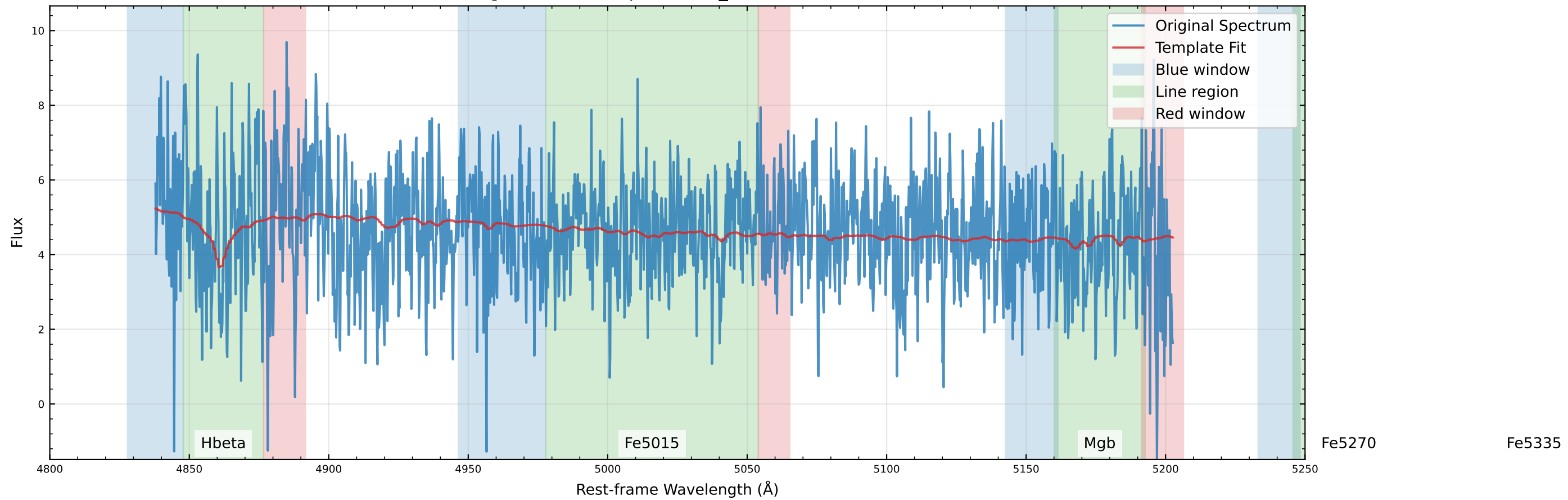
Original Data Comparison (v_star=-193.4 km/s)
