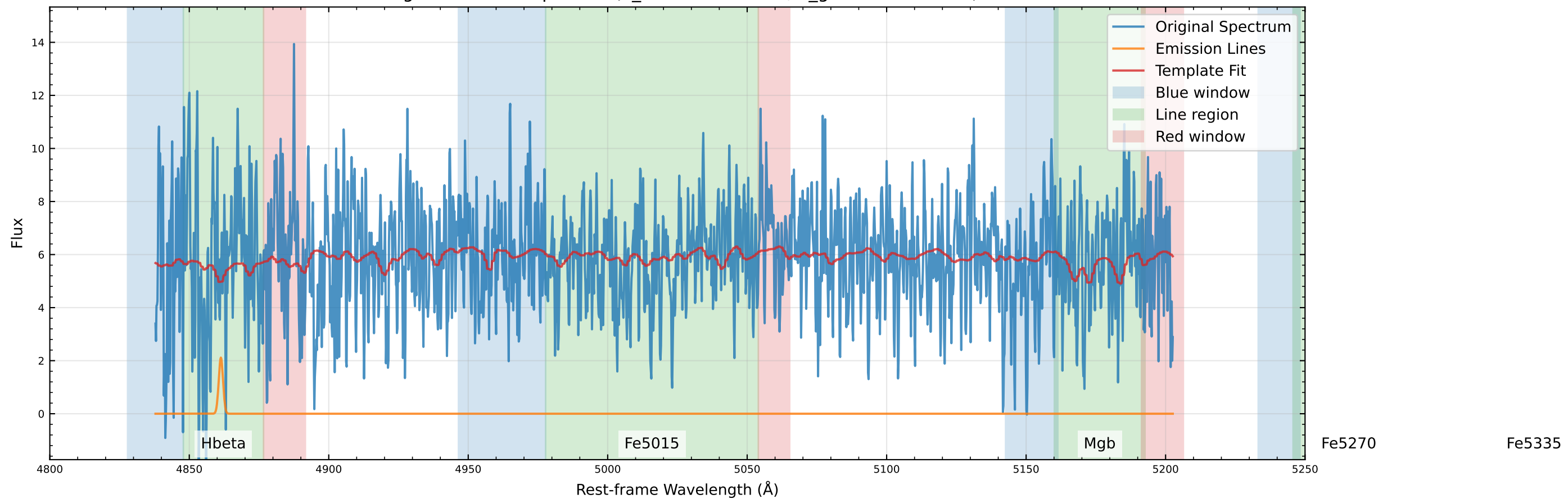
Original Data Comparison (v_star=-57.2 km/s, v_gas=-132.8 km/s)
