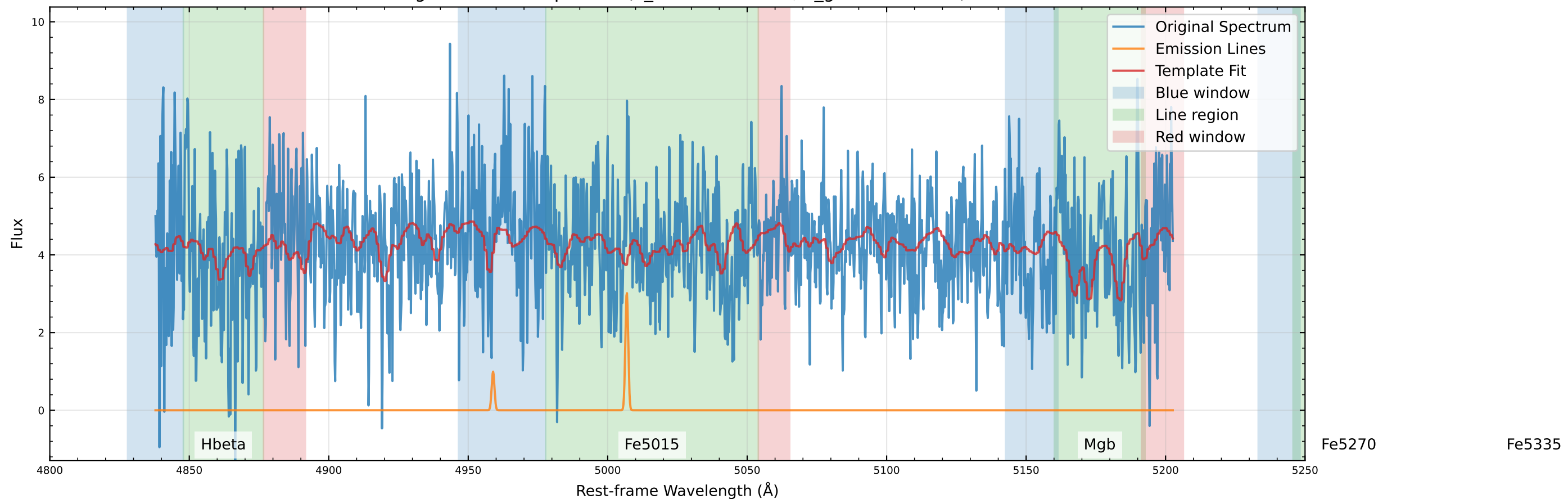
Original Data Comparison (v_star=77.2 km/s, v_gas=28.6 km/s)
