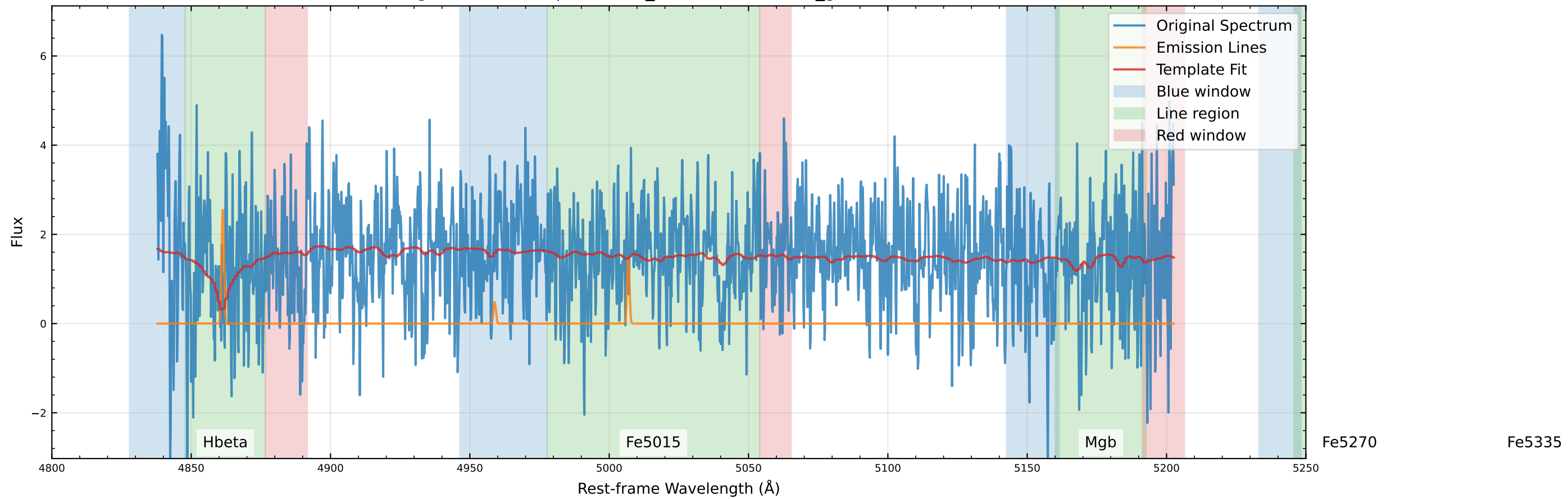
Original Data Comparison (v_star=84.6 km/s, v_gas=77.0 km/s)
