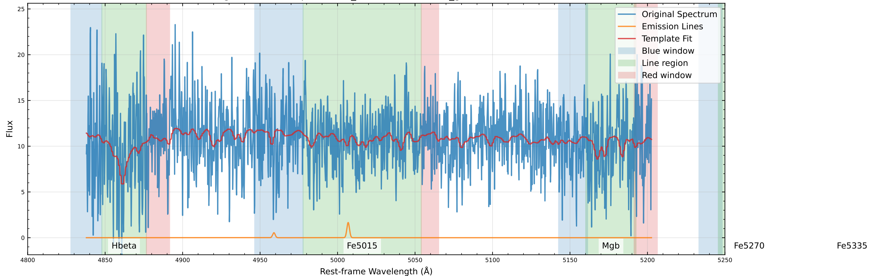
Original Data Comparison (v_star=-15.2 km/s, v_gas=-101.6 km/s)
