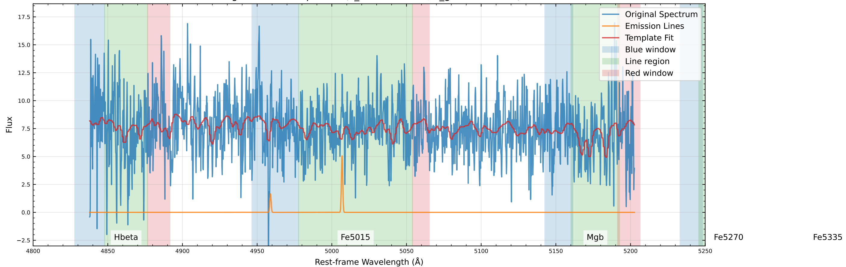
Original Data Comparison (v_star=6.2 km/s, v_gas=16.1 km/s)
