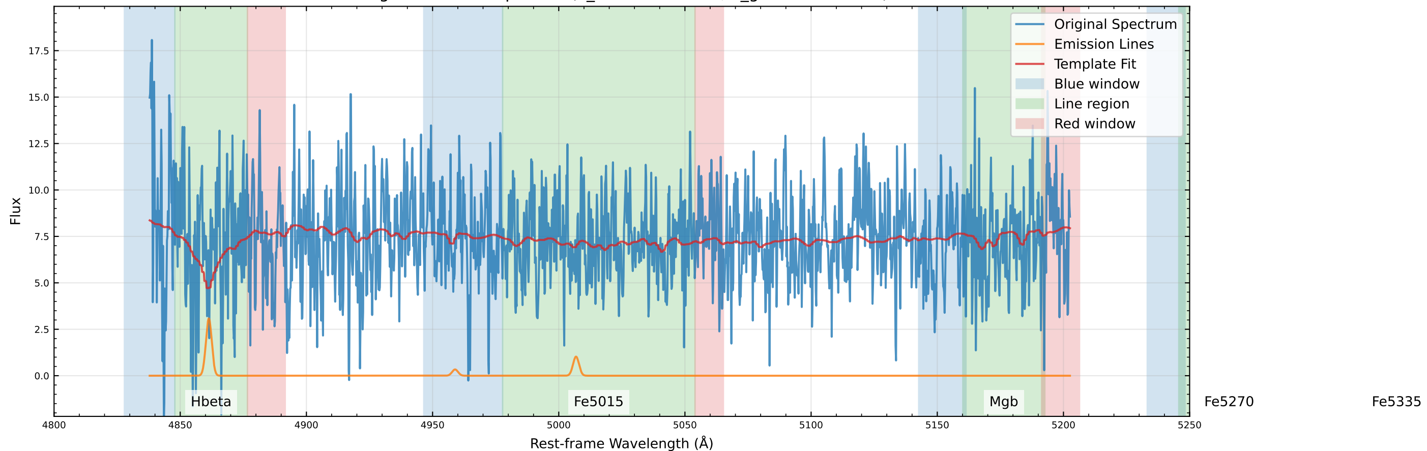
Original Data Comparison (v_star=68.8 km/s, v_gas=156.9 km/s)
