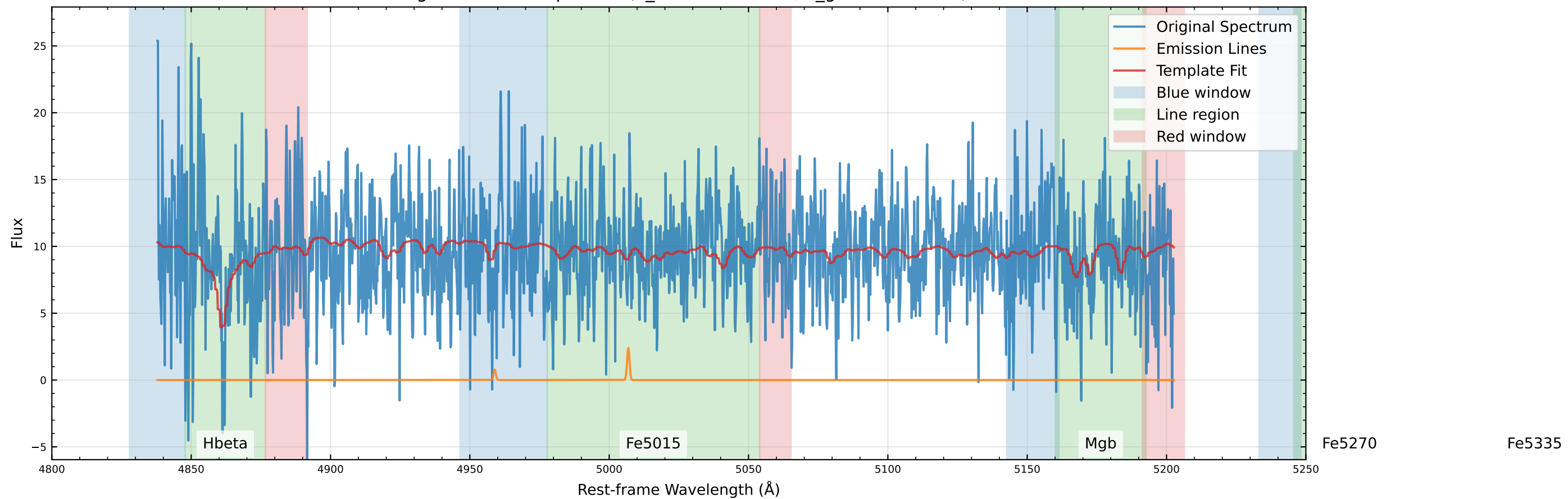
Original Data Comparison (v_star=22.2 km/s, v_gas=32.1 km/s)
