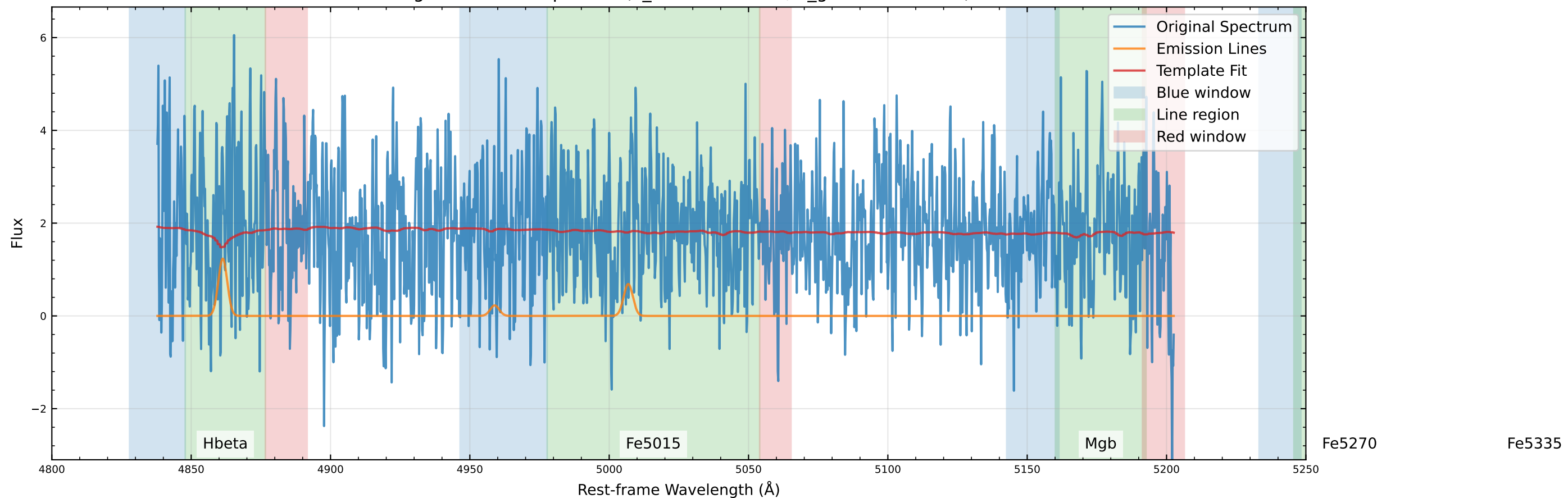
Original Data Comparison (v_star=-1.0 km/s, v_gas=149.0 km/s)
