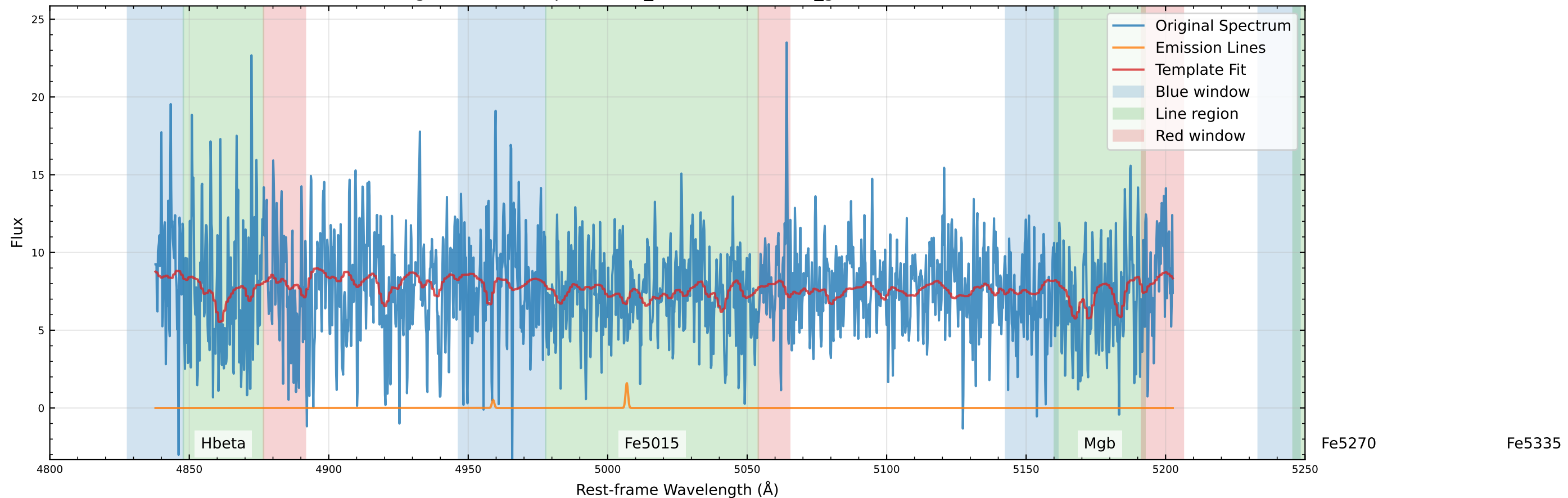
Original Data Comparison (v_star=50.1 km/s, v_gas=64.9 km/s)
