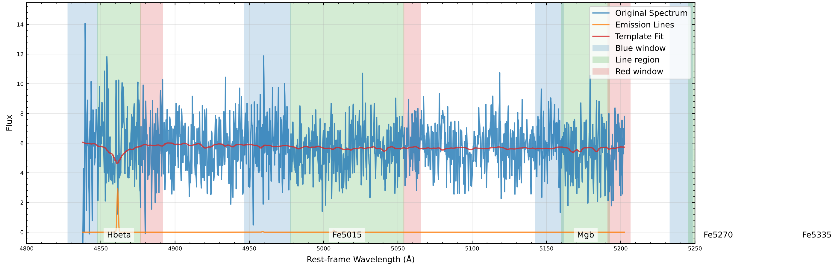
Original Data Comparison (v_star=-89.4 km/s, v_gas=-67.5 km/s)
