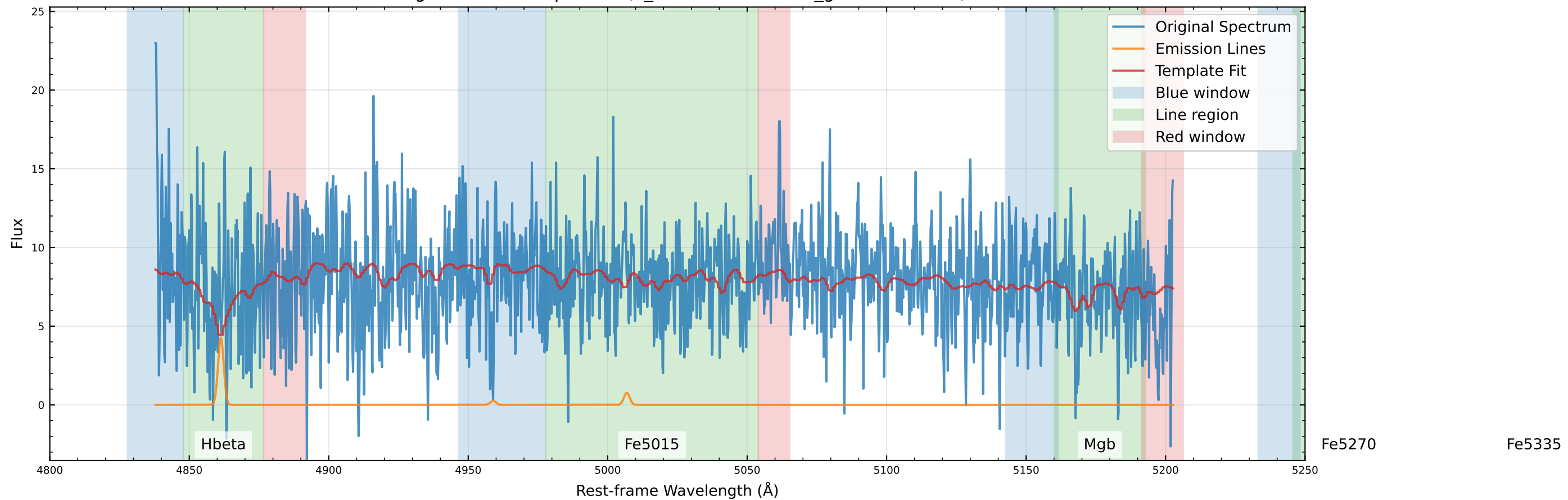
Original Data Comparison (v_star=33.5 km/s, v_gas=37.0 km/s)
