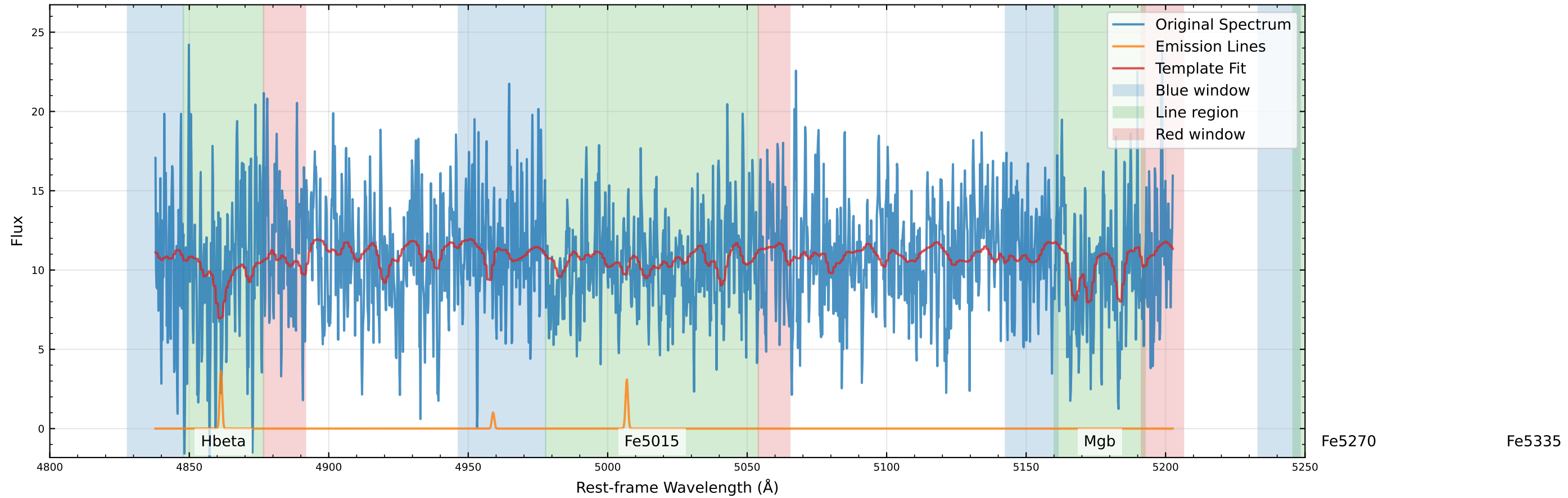
Original Data Comparison (v_star=-4.0 km/s, v_gas=-50.3 km/s)
