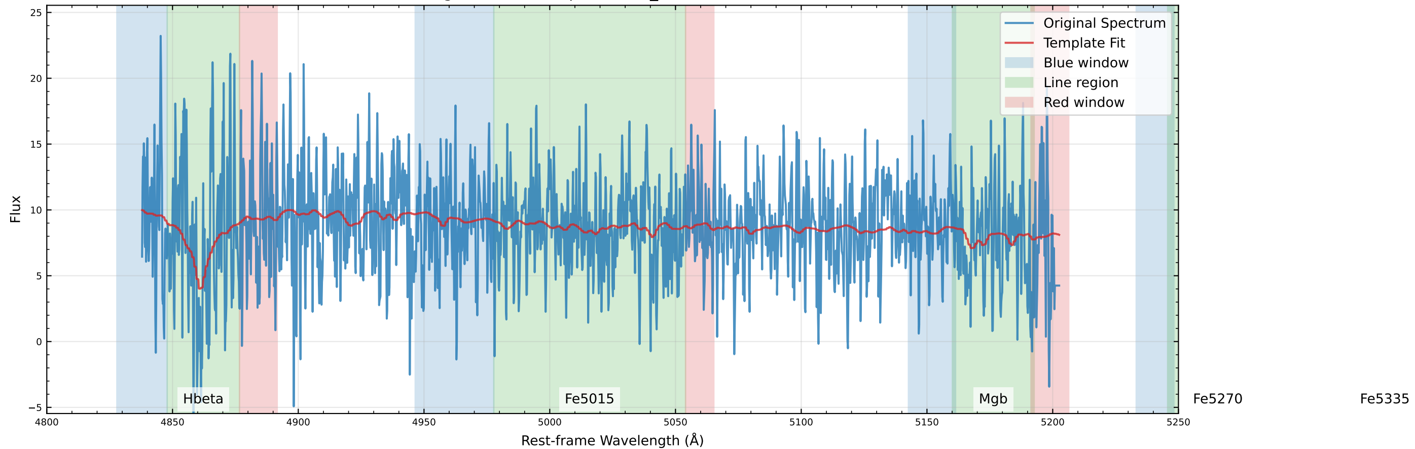
Original Data Comparison (v_star=-185.1 km/s)
