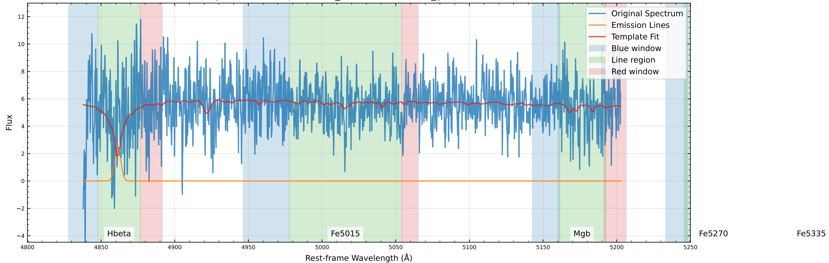
Original Data Comparison (v_star=240.4 km/s, v_gas=114.9 km/s)
