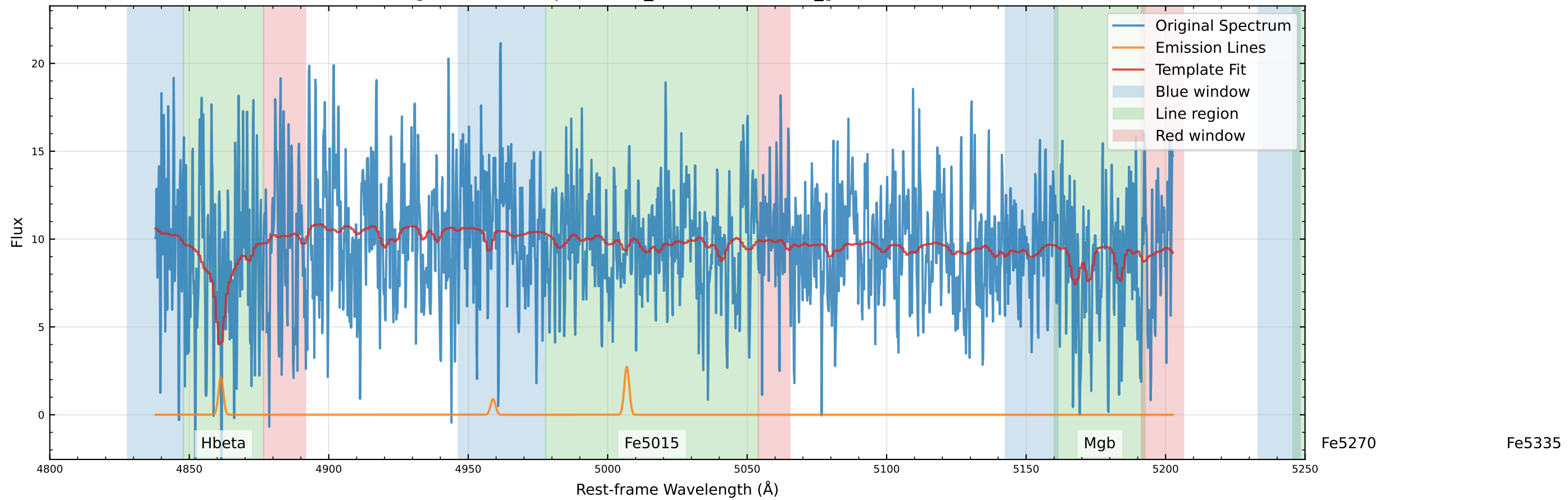
Original Data Comparison (v_star=34.1 km/s, v_gas=40.1 km/s)
