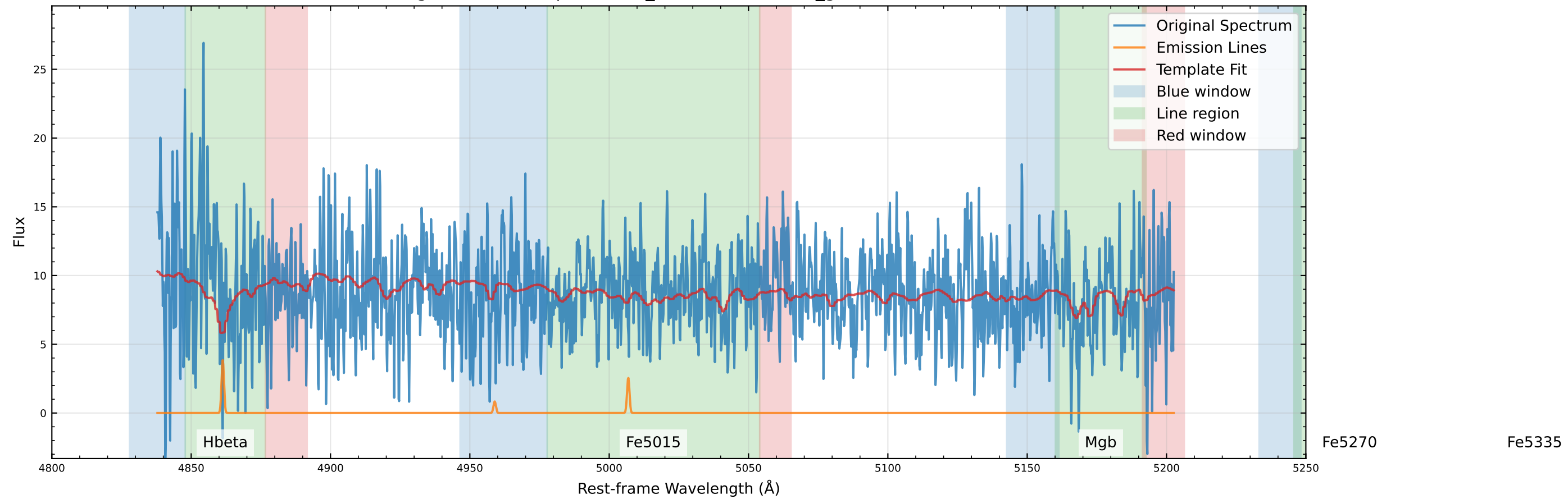
Original Data Comparison (v_star=49.5 km/s, v_gas=67.0 km/s)
