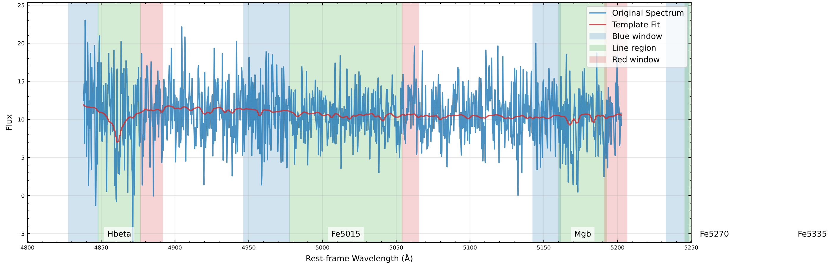
Original Data Comparison (v_star=35.8 km/s)
