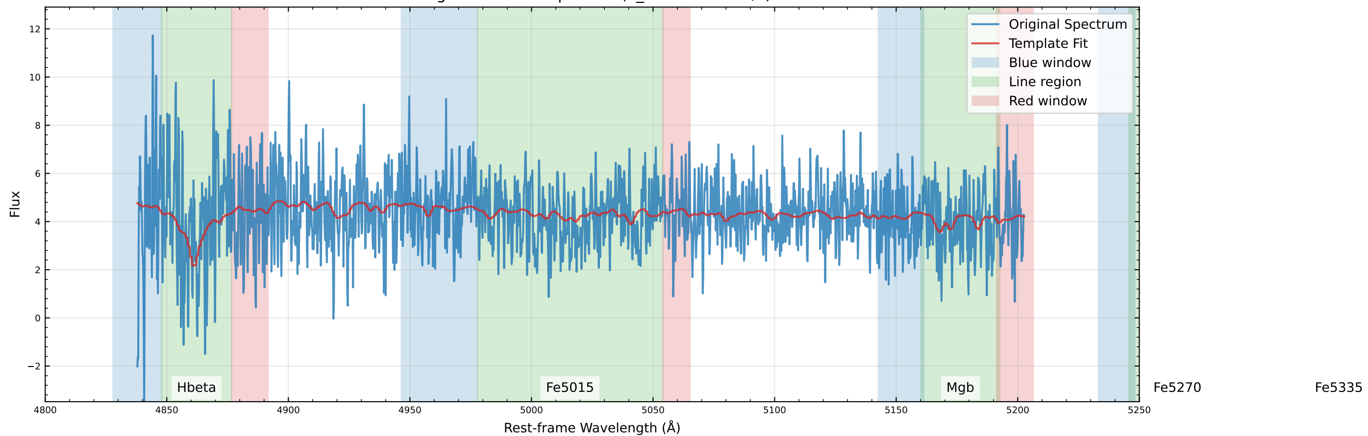
Original Data Comparison (v_star=43.8 km/s)
