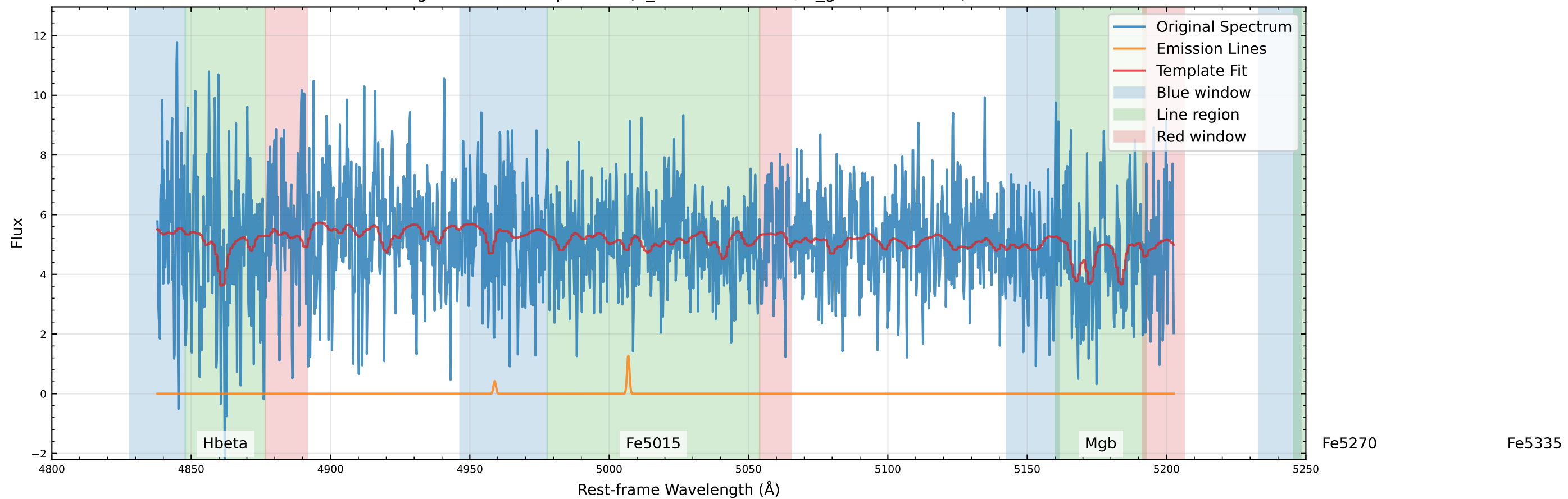
Original Data Comparison (v_star=34.0 km/s, v_gas=40.2 km/s)
