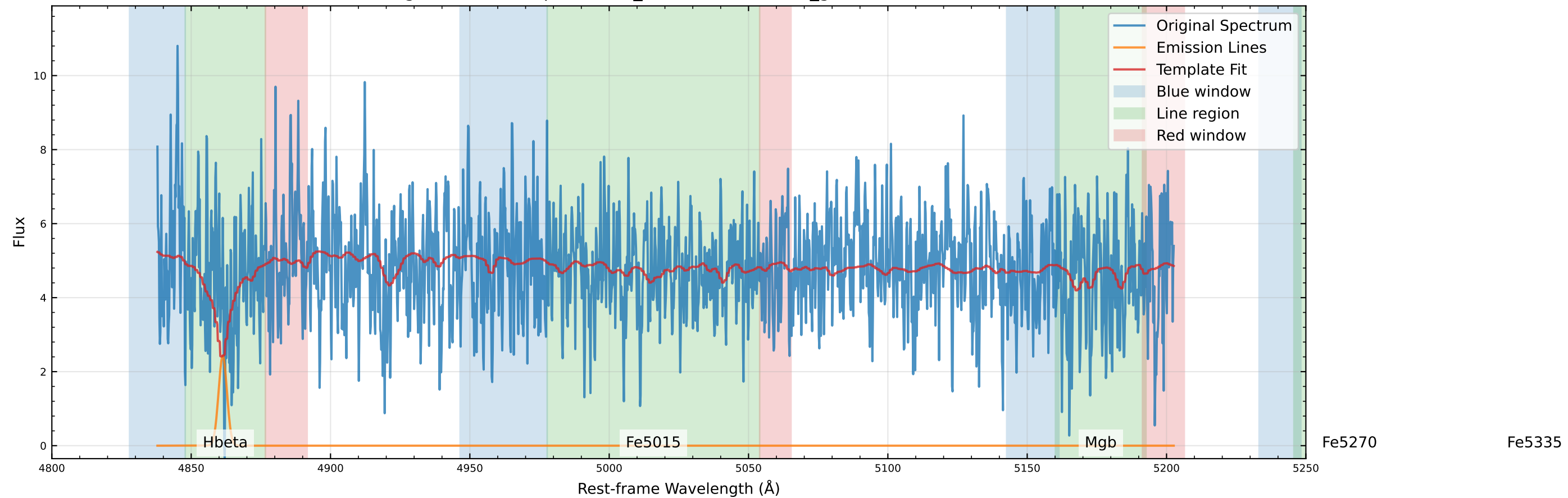
Original Data Comparison (v_star=-41.7 km/s, v_gas=-127.0 km/s)
