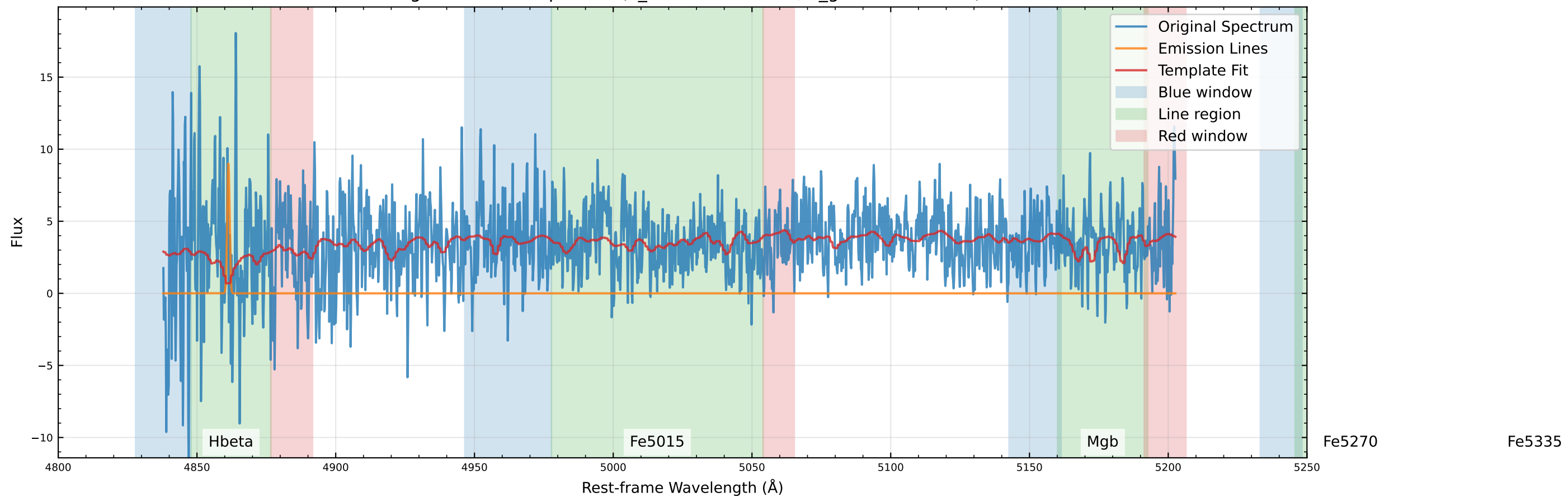
Original Data Comparison (v_star=171.4 km/s, v_gas=165.4 km/s)
