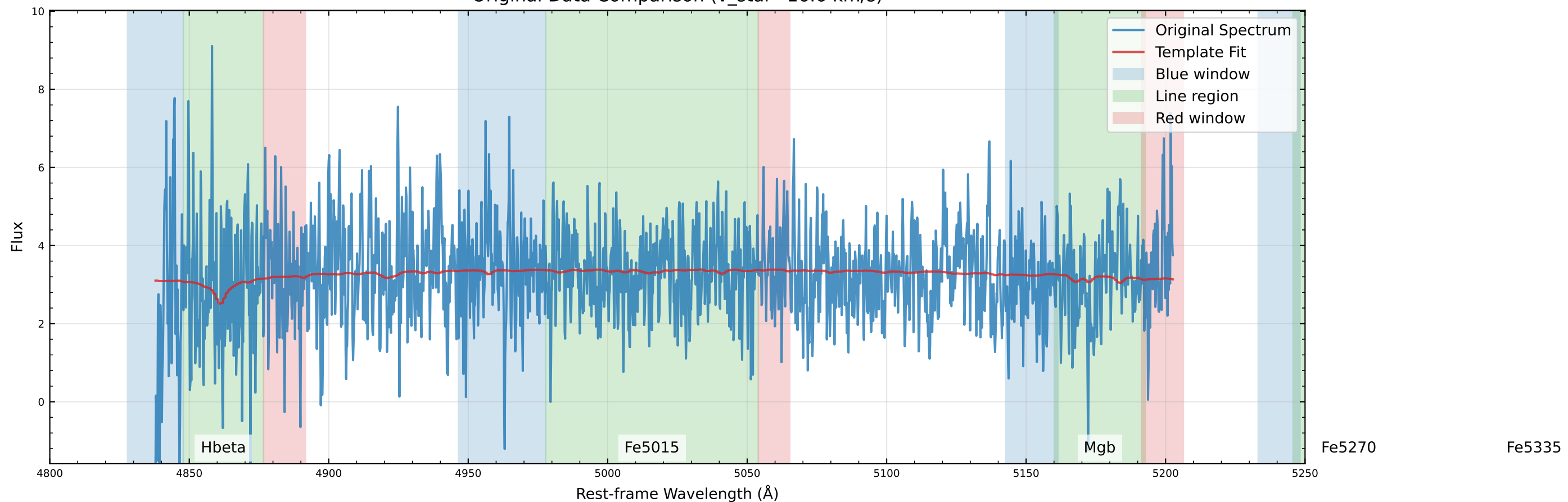
Original Data Comparison (v_star=16.6 km/s)
