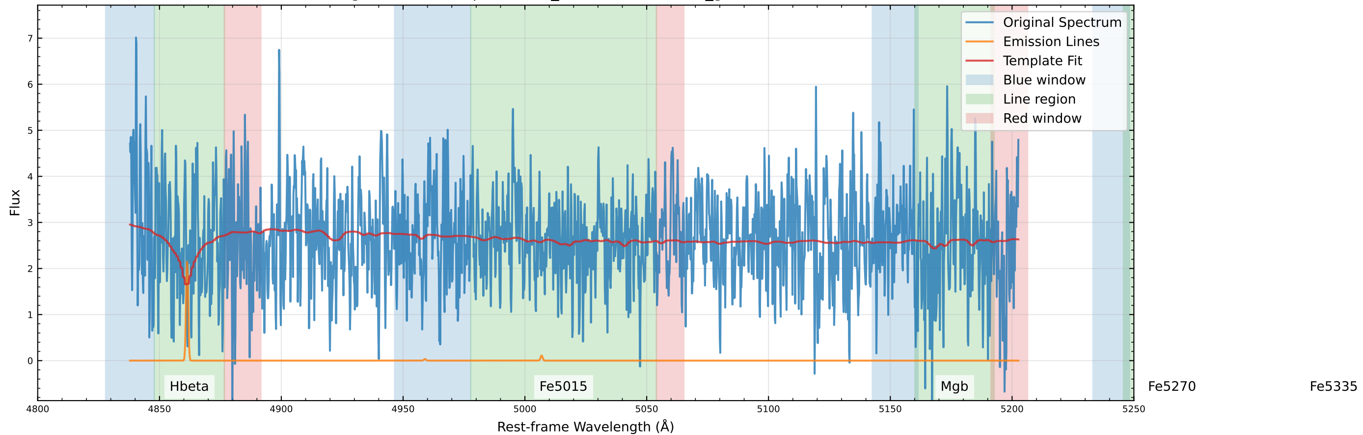
Original Data Comparison (v_star=-86.4 km/s, v_gas=-53.8 km/s)
