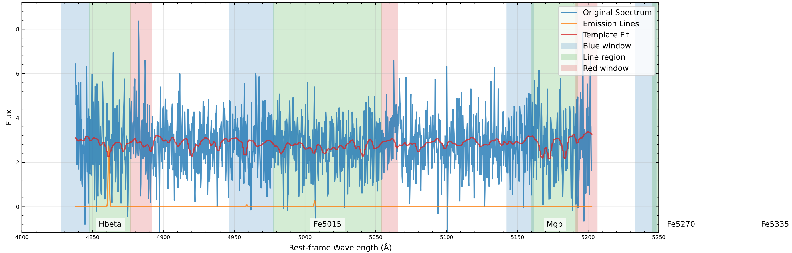
Original Data Comparison (v_star=237.2 km/s, v_gas=197.8 km/s)
