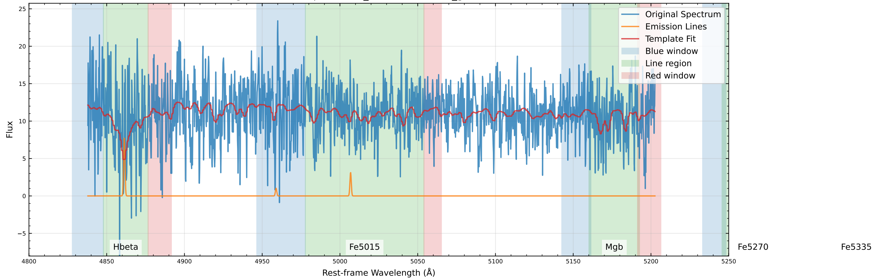
Original Data Comparison (v_star=1.8 km/s, v_gas=24.9 km/s)
