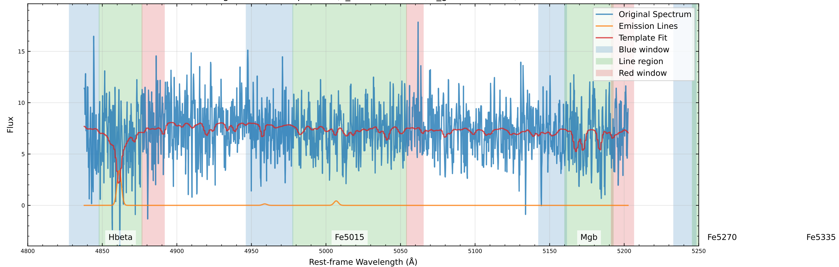
Original Data Comparison (v_star=52.7 km/s, v_gas=28.8 km/s)
