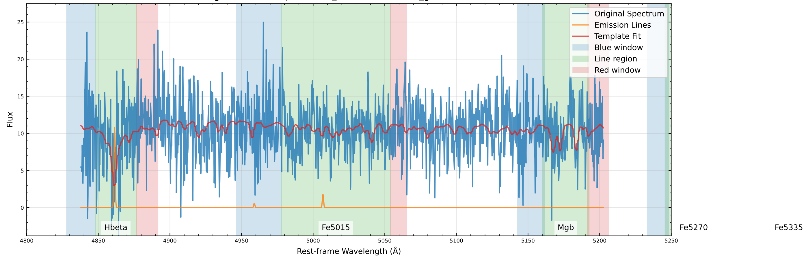
Original Data Comparison (v_star=56.0 km/s, v_gas=98.1 km/s)
