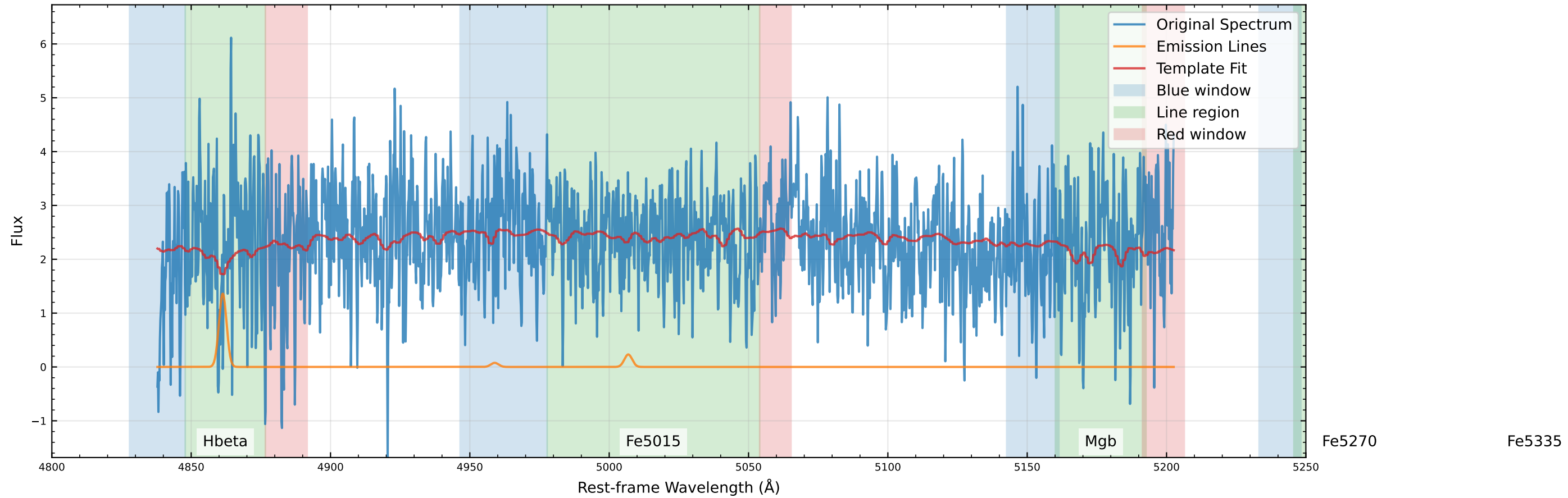
Original Data Comparison (v_star=34.9 km/s, v_gas=246.8 km/s)
