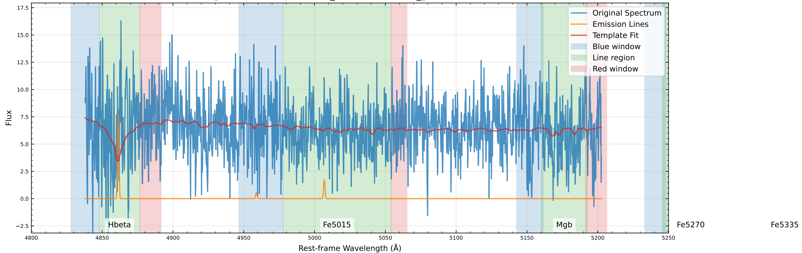
Original Data Comparison (v_star=24.5 km/s, v_gas=102.7 km/s)
